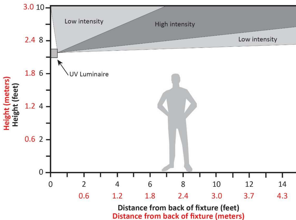
Figure 2-1. Upper-air GUV installation.
